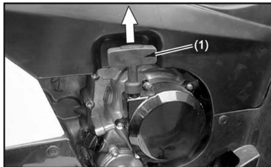
(1)手拉起動桿
